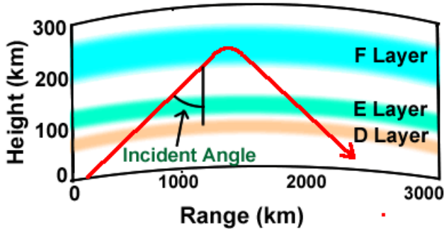
incident angle and refraction
