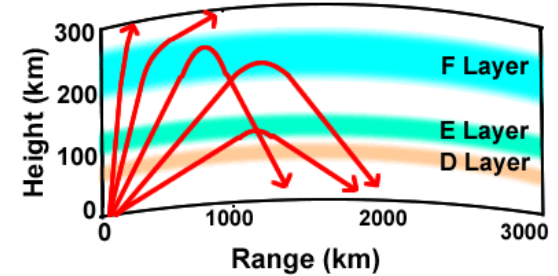
waves of the same frequency at several different transmission (and incident) angles
